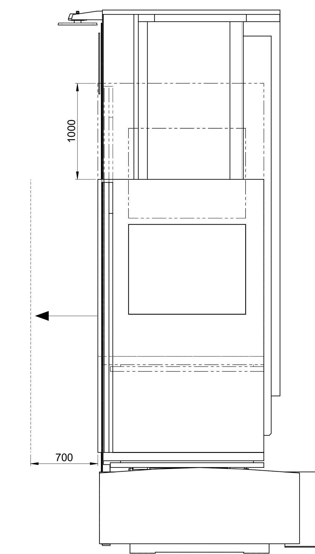
CORSE PEDANA OPERATORE OPERATOR PLATFORM'S STROKES
